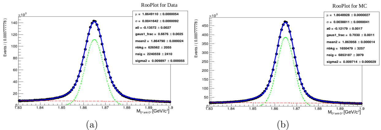
Figure 6: The fitted D^0\bar{D}^0 invariant mass distributions for Data (a) and MC (b) with double Gaussian + 1 st order of Chebyshev polynomial.
