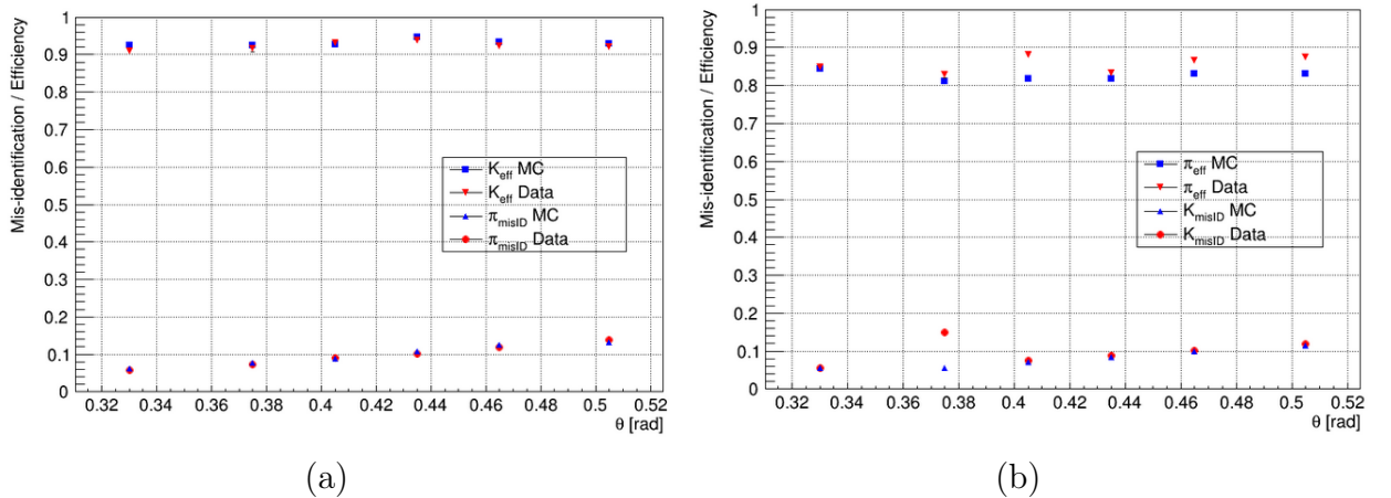
Figure 8: Efficiencies and mis-identification dependencies over polar angle binning.
