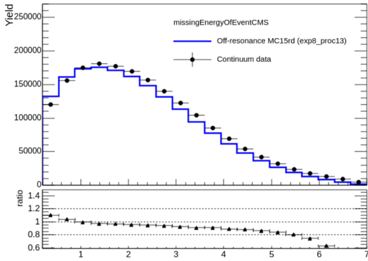
Figure 14: MissingEnergyOfEventCMS distribution before tuning.
