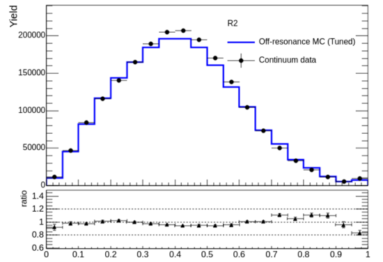
Figure 11: R_2 distribution after tuning.
