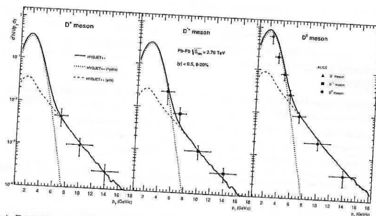
Figure 4: Transverse momentum spectra of D^\pm (left panel), D^\pm\pm (middle panel) and D^0 (right panel) for rapidity |y| < 0.5 in 20% of most central PbPb collisions at \sqrt{s_{NN}} = 2.76 TeV. The points denote ALICE data (see reference in the thesis), histograms represent simulated HYDJET++ events (blue dotted - soft component, red dashed - hard component, black solid - both components).
