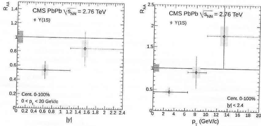
Figure 10: Nuclear modification factor R_{AA} of \Upsilon(1S) as a function of rapidity (left) and p_T (right). A global uncertainty of 8.3%, from T_{AA} and the integrated luminosity of the pp data sample, is shown as a grey box at R_{AA} = 1 . Points are plotted at their measured average p_T . Statistical (systematic) uncertainties are shown as bars (boxes). Horizontal bars indicate the bin width.
