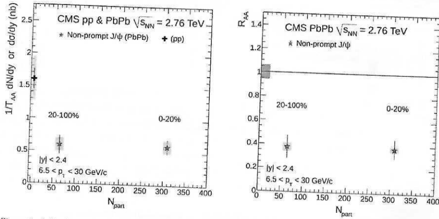
Figure 9: Left: Non-prompt J/\psi yield in PbPb collisions divided by T_{AA} compared to the pp cross-section. Right: Nuclear modification factor R_{AA} of non-prompt J/\psi as a function of N_{part} . A global uncertainty of 6%, from the integrated luminosity of the pp data sample, is shown as a grey box at R_{AA} = 1 .
