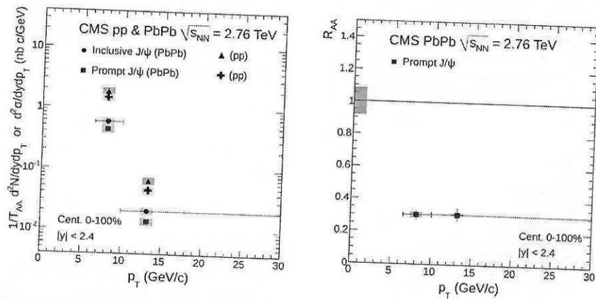
Figure 7: Left: yield of inclusive J/\psi (blue circles) and prompt J/\psi (red squares) divided by T_{AA} as a function of p_T . The results are compared to the cross sections of inclusive J/\psi (black triangles) and prompt J/\psi (black crosses) measured in pp . The global scale uncertainties on the PbPb data due to T_{AA} (5.7%) and the pp integrated luminosity (6.0%) are not shown. Right: nuclear modification factor R_{AA} of prompt J/\psi as a function of p_T . A global uncertainty of 8.3%, from T_{AA} and the integrated luminosity of the pp data sample, is shown as a grey box at R_{AA} = 1 . Points are plotted at their measured average p_T . Statistical (systematic) uncertainties are shown as bars (boxes). Horizontal bars indicate the bin width.
