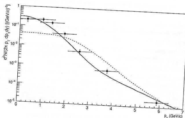
Figure 5: Transverse-momentum distribution of D^0 mesons in 10% of the most central Au-Au collisions at the energy \sqrt{s_{NN}} = 200 GeV for the rapidity range |y| < 1 . The points are STAR data from (see reference in the thesis) and the lines are the results of the HYDJET++ simulation with the freeze-out parameters for inclusive hadrons (red dashed line) and "early" thermal freeze-out (solid blue line).
