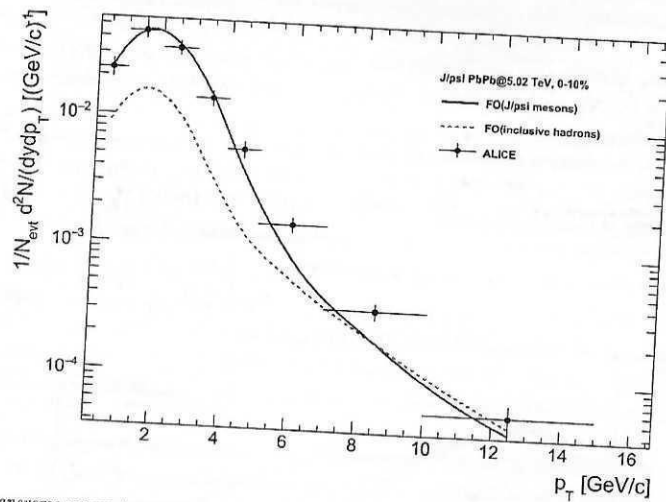
Figure 3: Transverse momentum spectrum of inclusive J/\psi -mesons for rapidity |y| < 0.9 in 10% of most central PbPb collisions at \sqrt{s_{NN}} = 5.02 TeV. The points denote ALICE data (see reference in the thesis), histograms represent simulated HYDJET++ events (red dashed - freeze-out parameters as for inclusive hadrons, blue solid - early thermal freeze-out).
