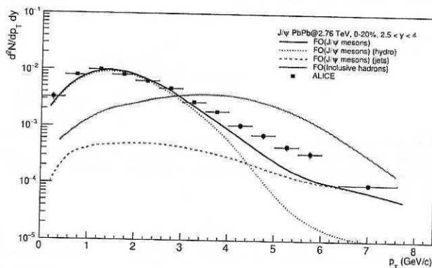
Figure 2: Transverse momentum spectrum of inclusive J/\psi -mesons for rapidity 2.5 < y < 4 in 20% of most central PbPb collisions at \sqrt{s_{NN}} = 2.76 TeV. The points denote ALICE data (reference in the thesis), histograms represent simulated HYDJET++ events (magenta solid - freeze-out parameters as for inclusive hadrons, black solid - early thermal freeze-out, blue dotted and red dashed - soft and hard components respectively for the latter case).
