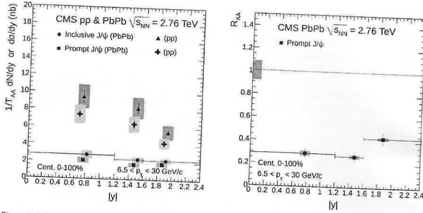
Figure 8: Left: yield of inclusive J/\psi (blue circles) and prompt J/\psi (red squares) divided by T_{AA} as a function of rapidity. The results are compared to the cross sections of inclusive J/\psi (black triangles) and prompt J/\psi (black crosses) measured in pp. The inclusive J/\psi points are shifted by \Delta y = 0.05 for better visibility. The global scale uncertainties on the PbPb data due to T_{AA} (5.7%) and the pp integrated luminosity (6.0%) are not shown. Right: nuclear modification factor R_{AA} of prompt J/\psi as a function of rapidity. A global uncertainty of 8.3%, from T_{AA} and the integrated luminosity of the pp data sample, is shown as a grey box at R_{AA} = 1 . Points are plotted at their measured average |y| . Statistical (systematic) uncertainties are shown as bars (boxes). Horizontal bars indicate the bin width.
